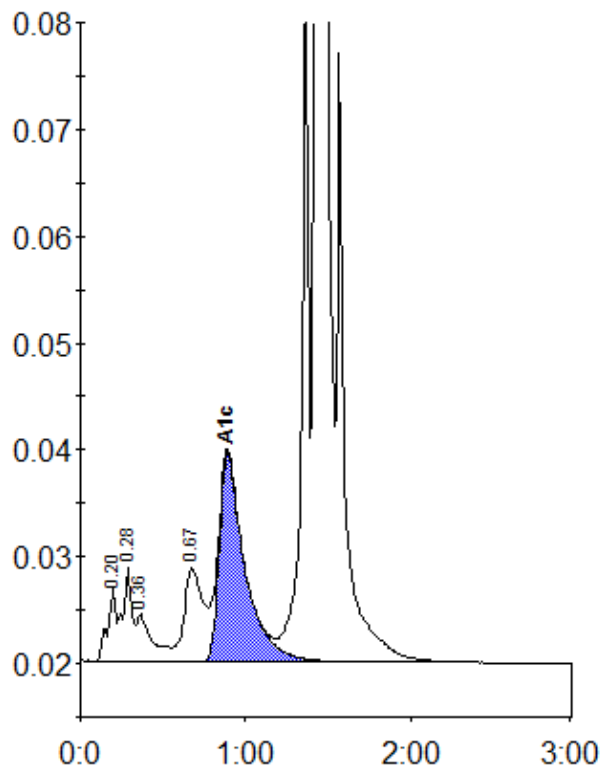
Peak table - ID: 10347307
